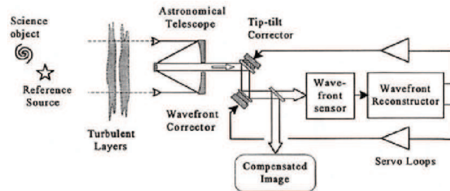
FIGURE 12. Astronomical Adaptive Optics System
