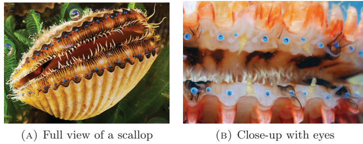
FIGURE 4. Scallop with hundreds of eyes
