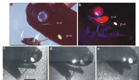
FIGURE 7. Stoptlight Loosejaw uses bioluminescence from 2 spots
