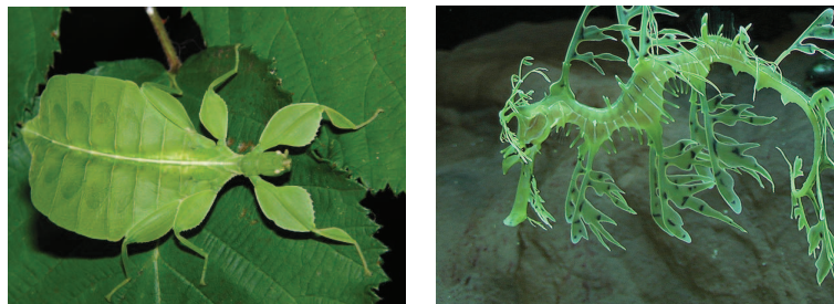
(A) Leaf insect
