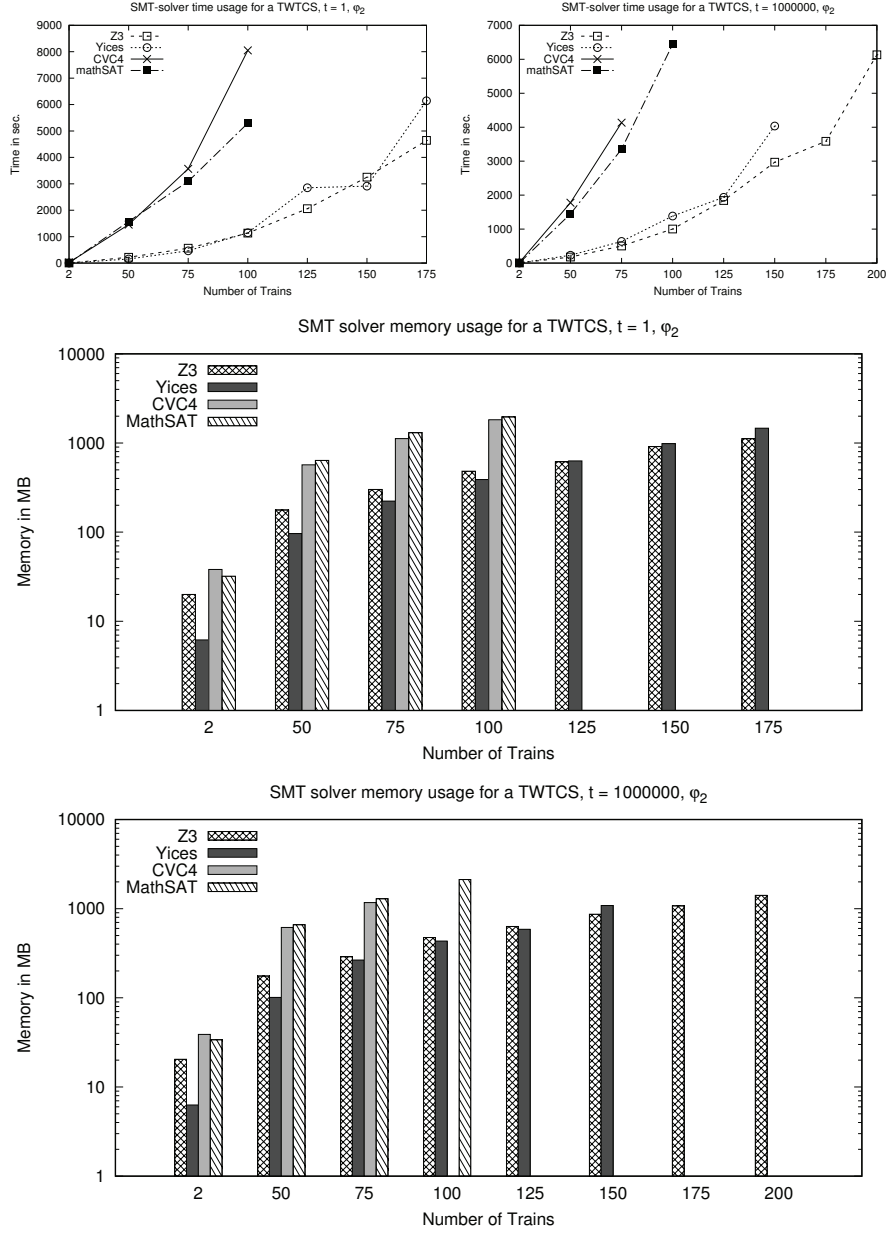
FIGURE 7. SMT-based BMC: TWTCs with n trains.
